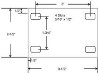
ENDW3 Water Line Adapter (ENDW2 & ENDW1)
