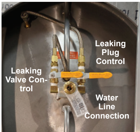
Manifold View
