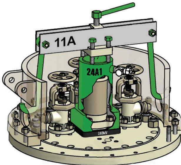
Device 24 Showing Yoke Assembly 11A installed with Device 24
