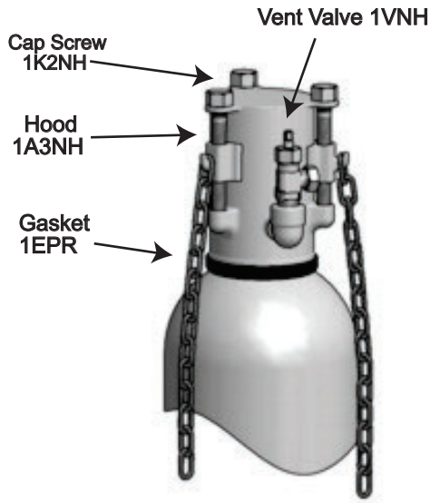
AMMONIA Cylinder DOT 3AA480
